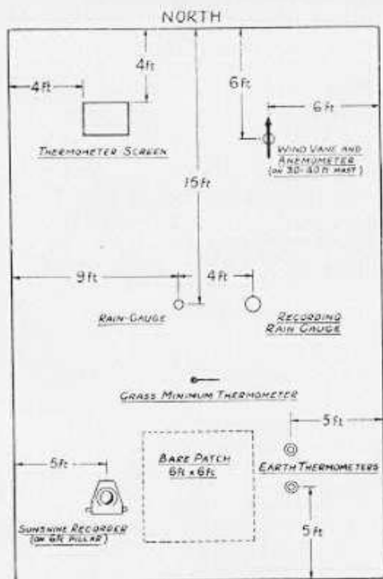
Recommended Layout of a Meteorological Station
